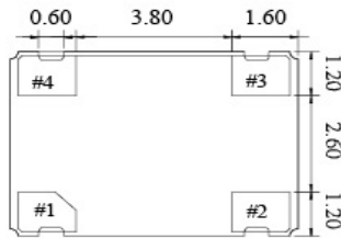
Recommended Solder Pattern
