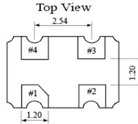
Recommended Solder Pattern
